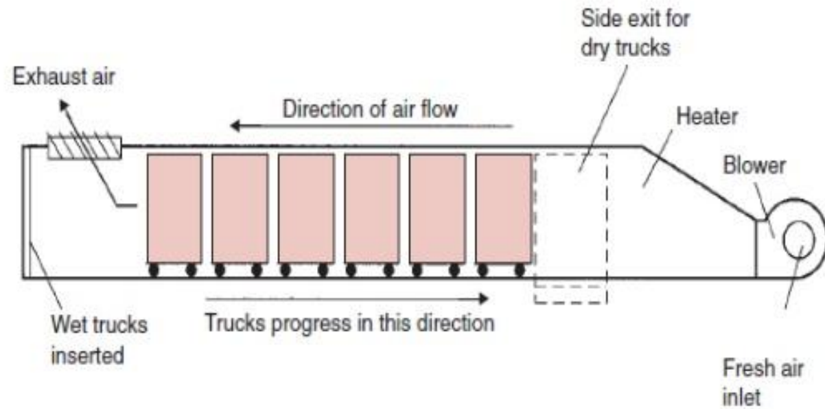
Fig. 12.7 Schematic of a counter current-flow tunnel dryer. [From Van Arsdel (1951).]
